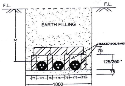
LAYING OF 3 NOS CABLES IN TRENCH
