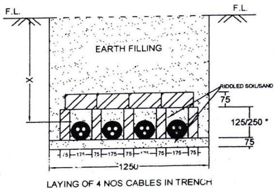
LAYING OF 4 NOS CABLES IN TRENCH
